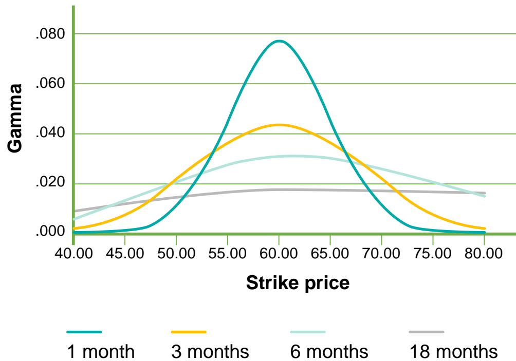
Gamma vs. time
