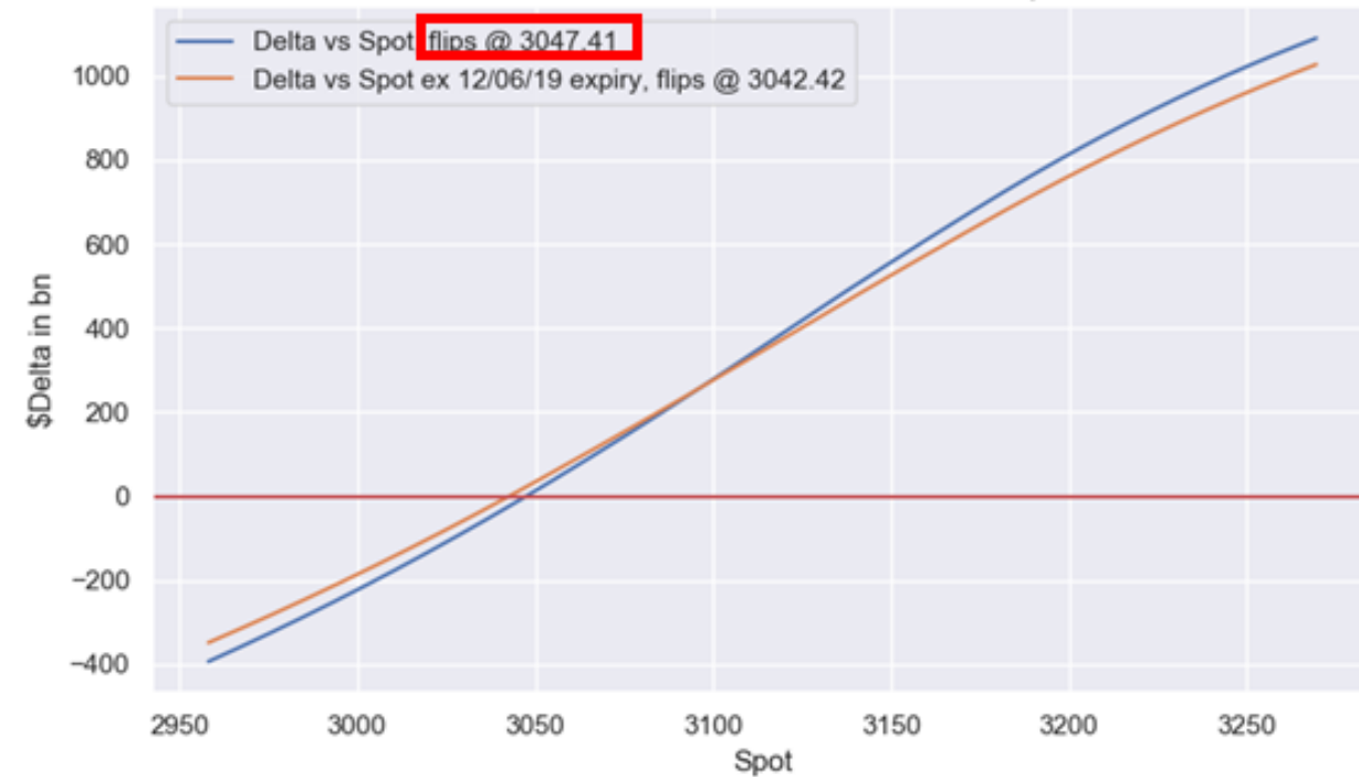
SPX and SPY Combined Delta vs Spot
